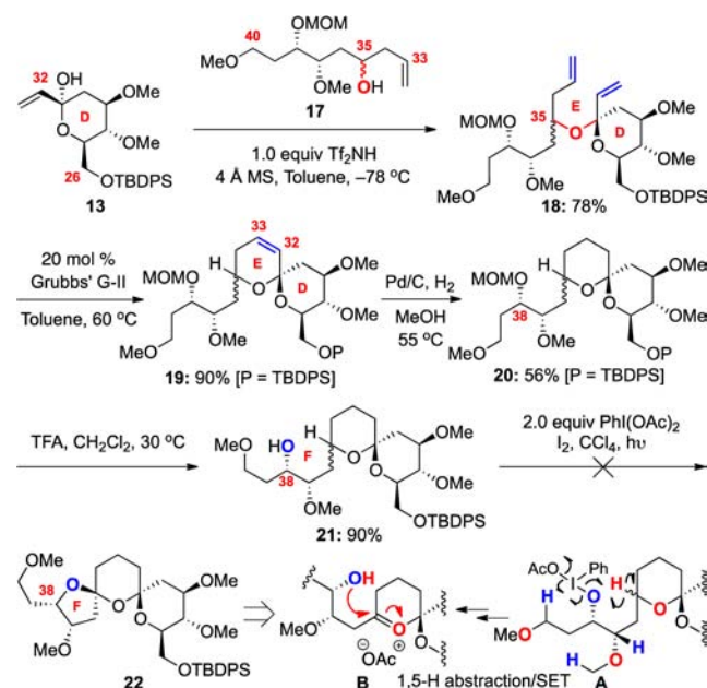
Scheme 5. Attempted Cyclic Acetal Tethered RCM–Suárez Oxidative Cyclization Sequence
